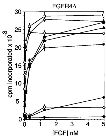
FIG. 5. BaF3 cell mitogenic assays using cells expressing the two Ig-like domain form of FGFR 4. The symbols used to represent FGFs are the same as those shown in Fig. 2.
